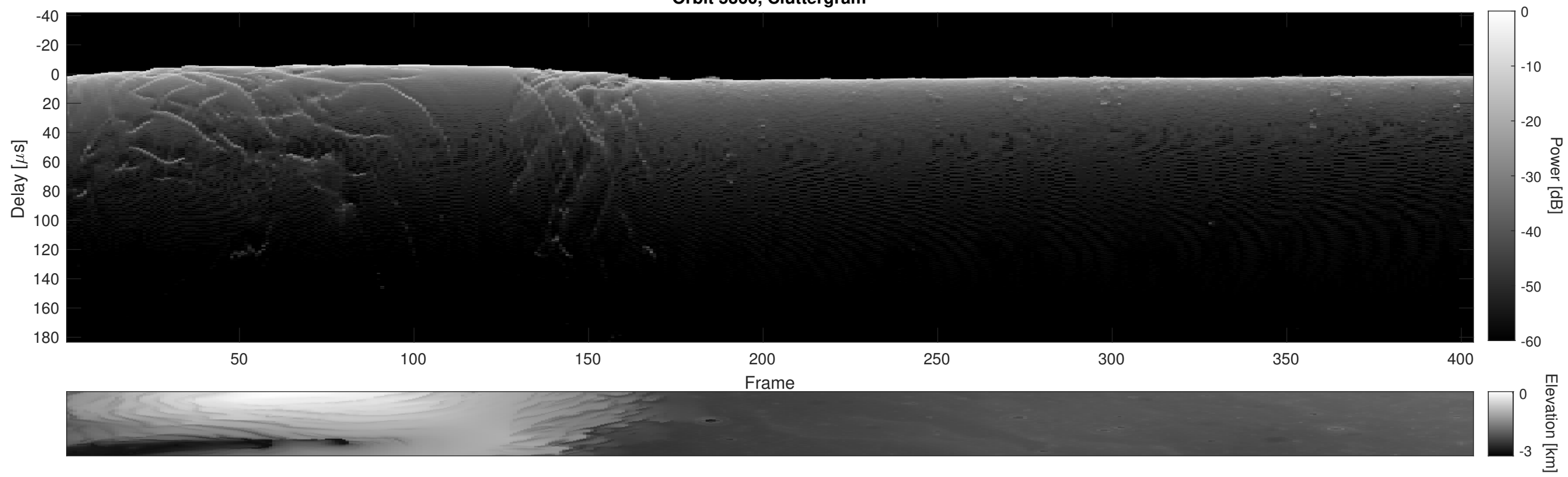
Orbit 5360, Cluttergram
