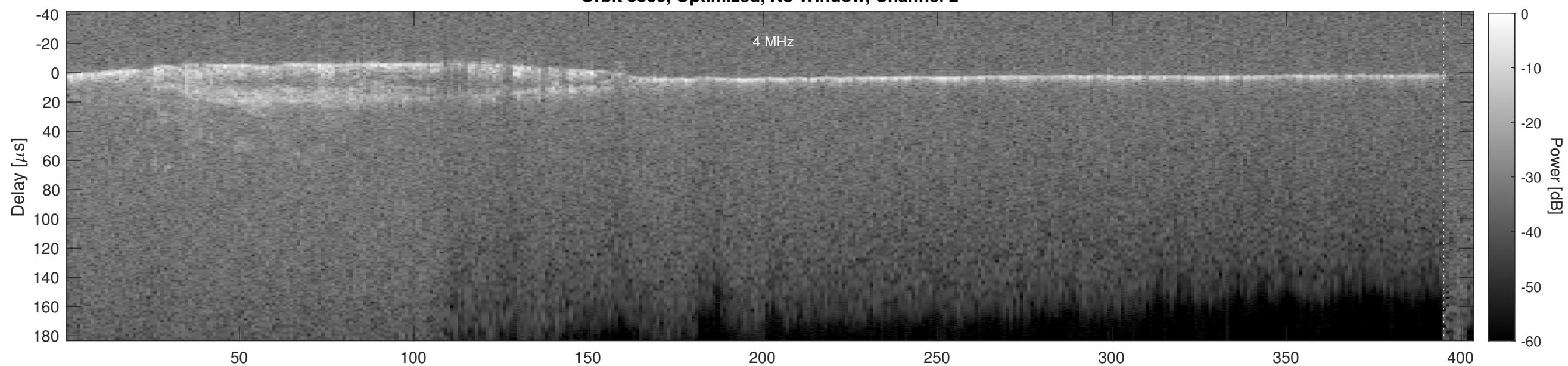
Orbit 5360, Cluttergram
