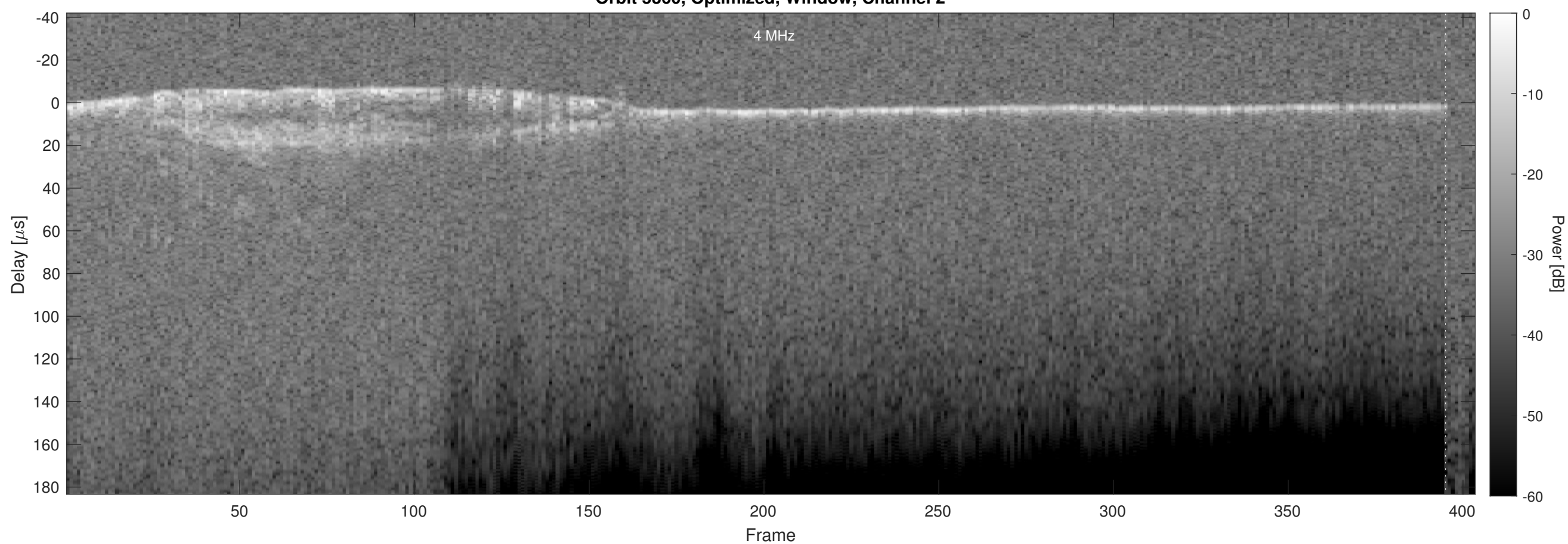
Orbit 5360, Optimized, Window, Channel 2
