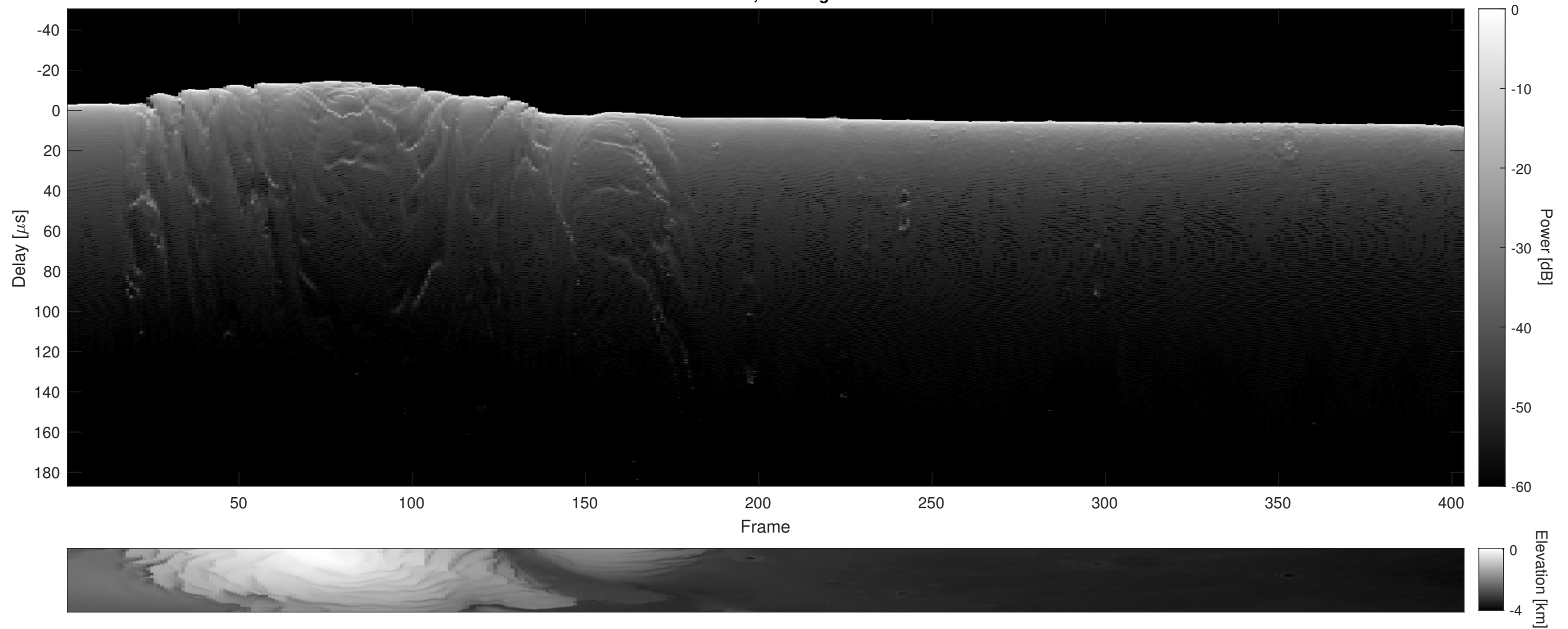
Orbit 5361, Cluttergram
