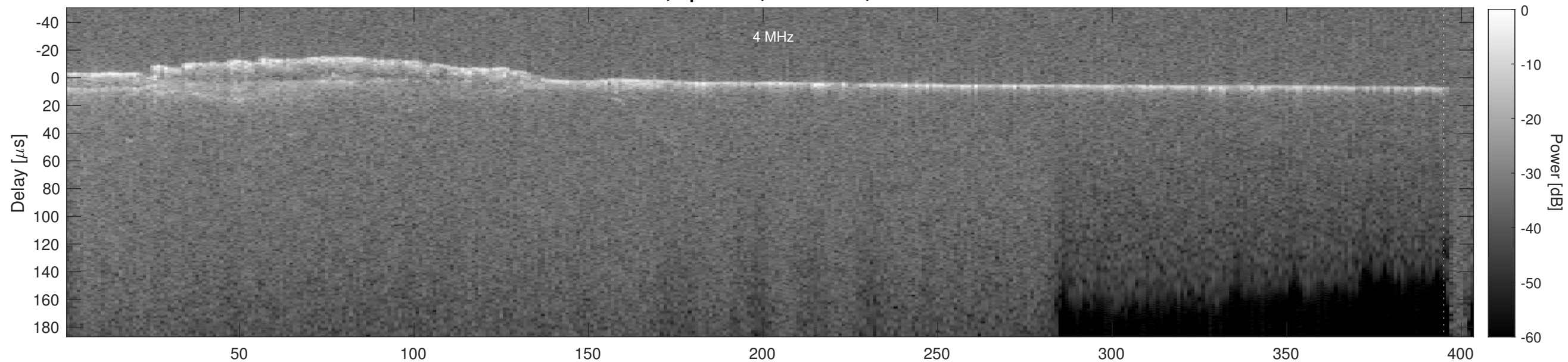
Orbit 5361, Cluttergram
