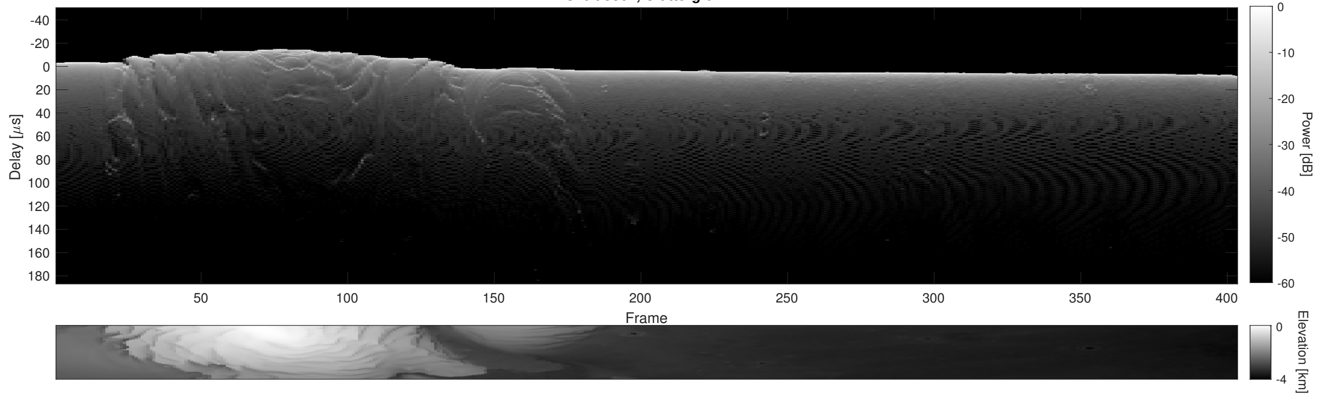
Orbit 5361, Cluttergram
