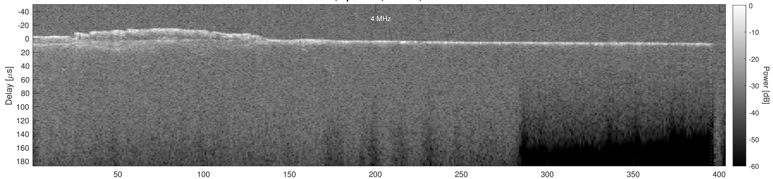
Orbit 5361, Cluttergram
