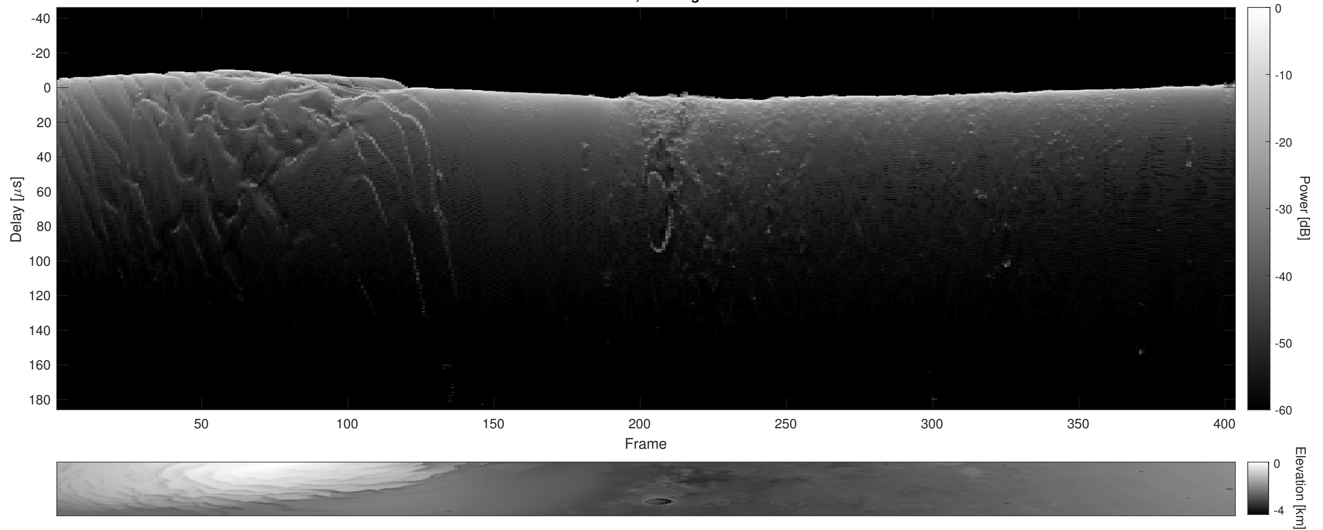
Orbit 5362, Cluttergram
