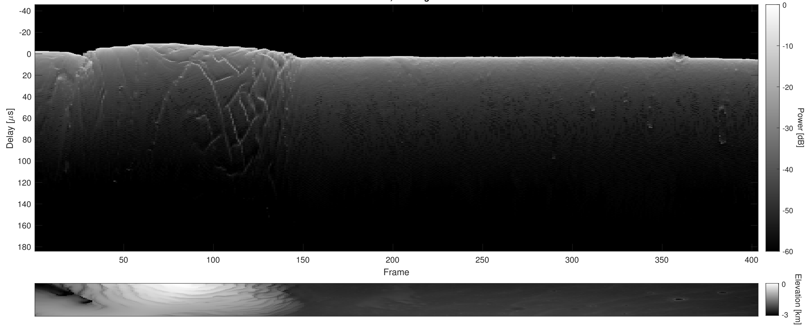
Orbit 5363, Cluttergram
