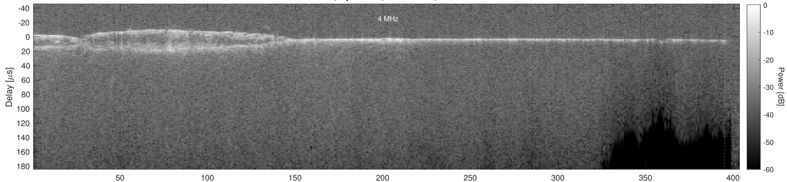
Orbit 5363, Cluttergram
