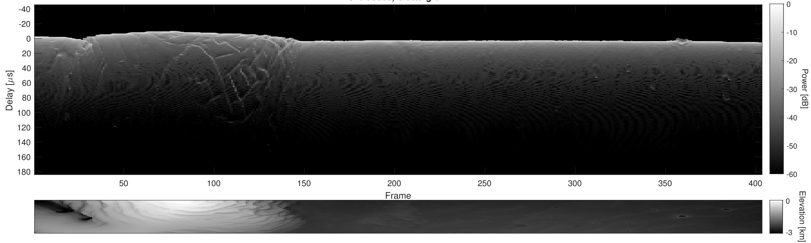
Orbit 5363, Cluttergram
