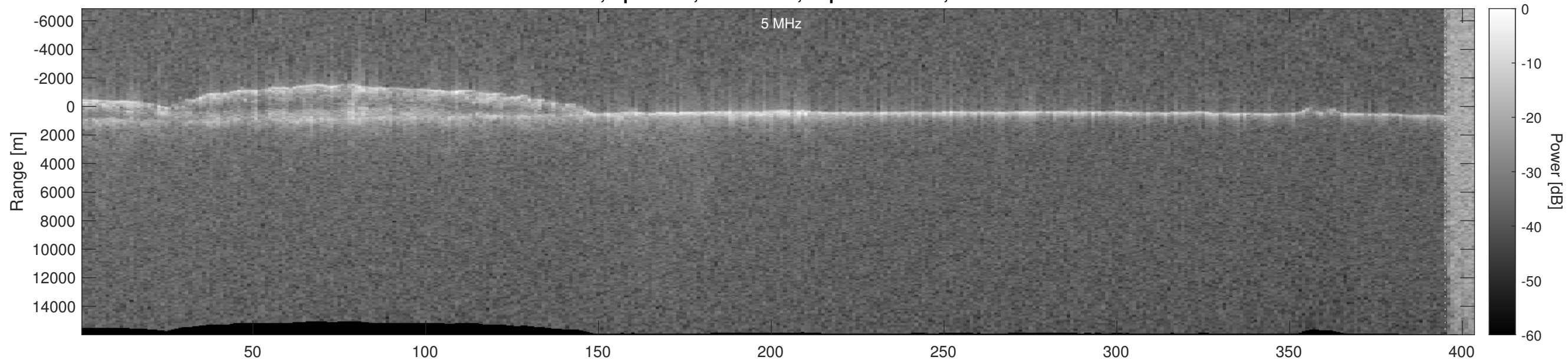
Orbit 5363, Optimized, No Window, Depth-Corrected, Channel 2
