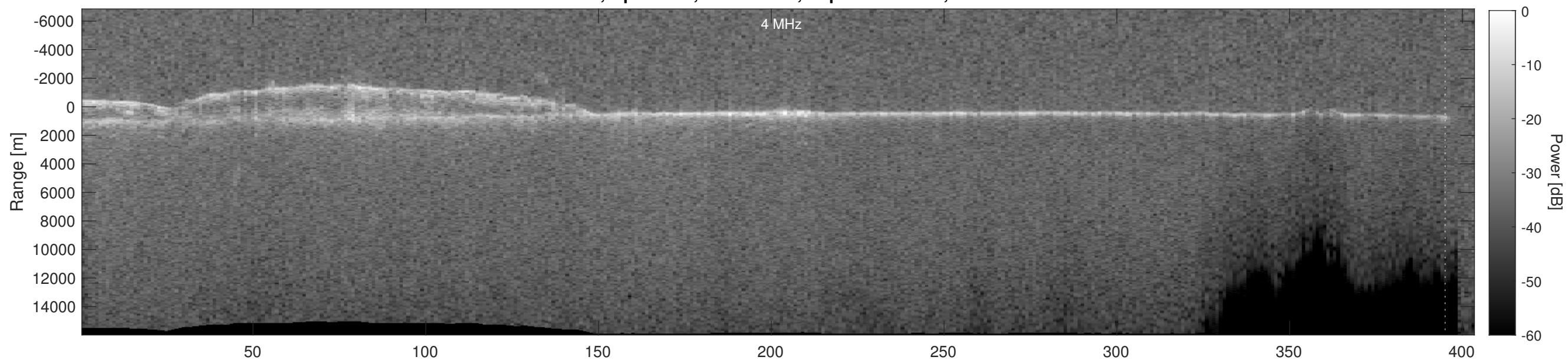
Orbit 5363, Depth-Corrected Cluttergram
