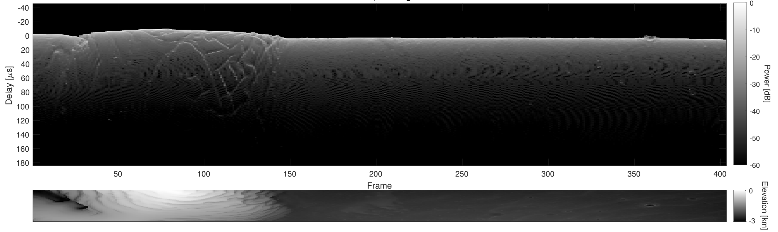
Orbit 5363, Cluttergram
