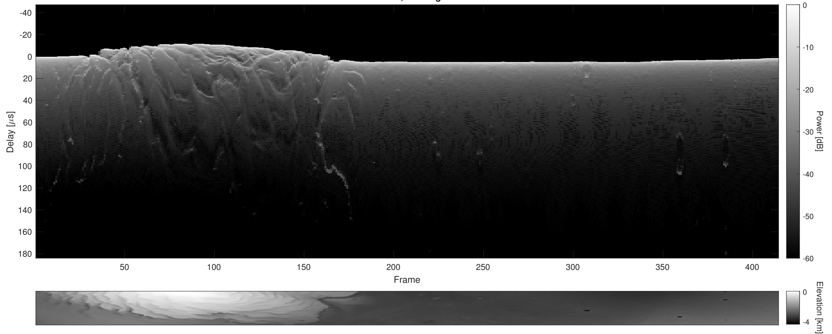
Orbit 5365, Cluttergram
