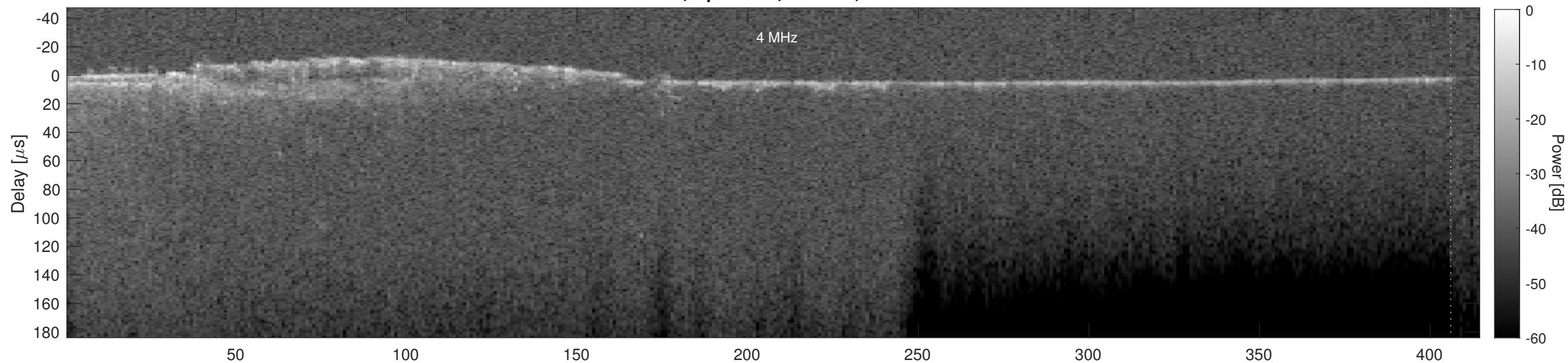
Orbit 5365, Cluttergram
