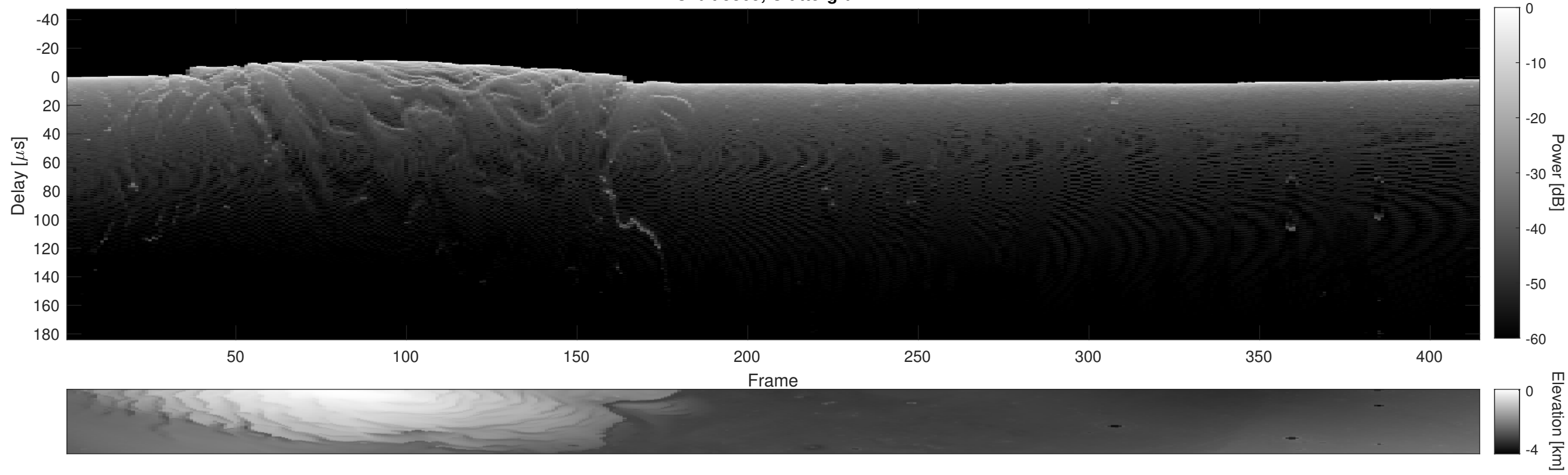
Orbit 5365, Cluttergram
