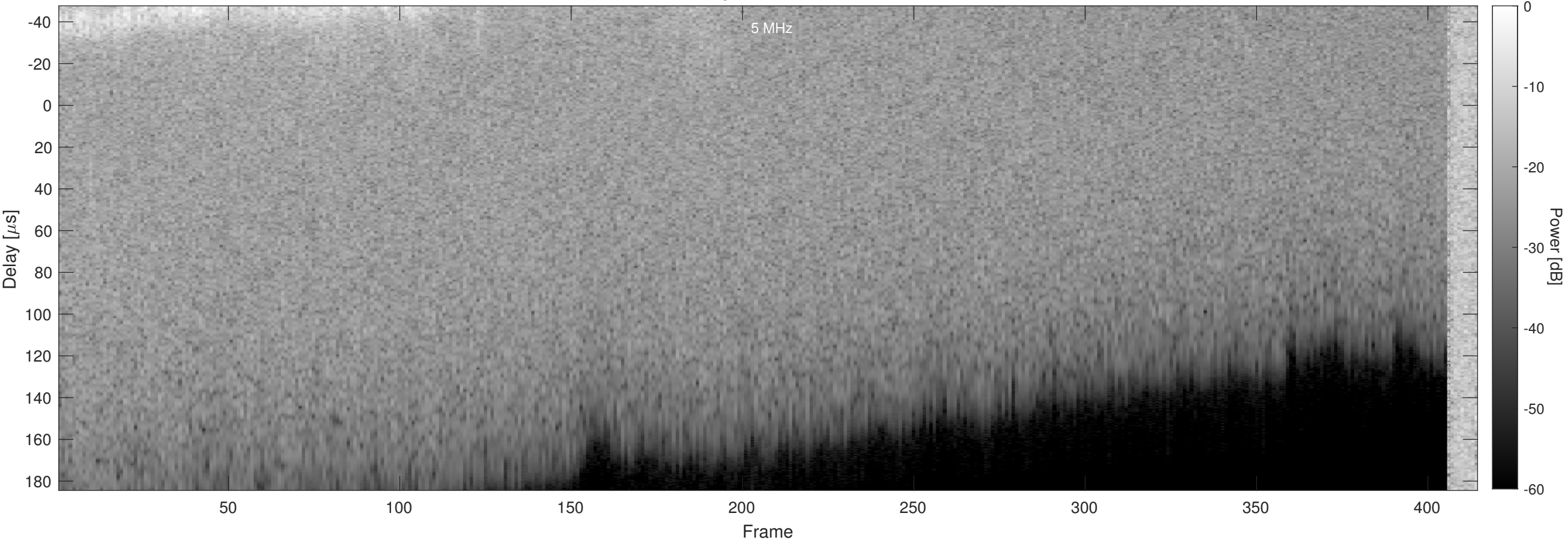
Orbit 5366, Chapman, Window, Channel 2
