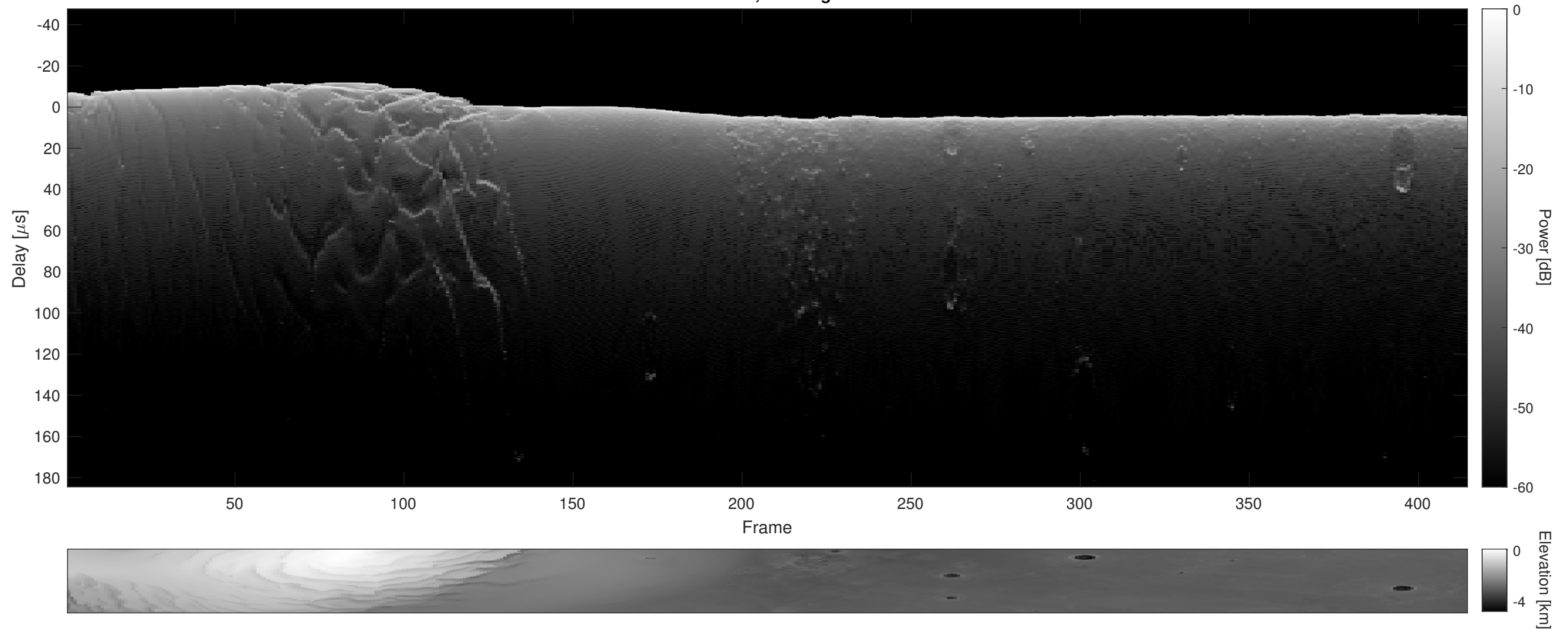
Orbit 5366, Cluttergram
