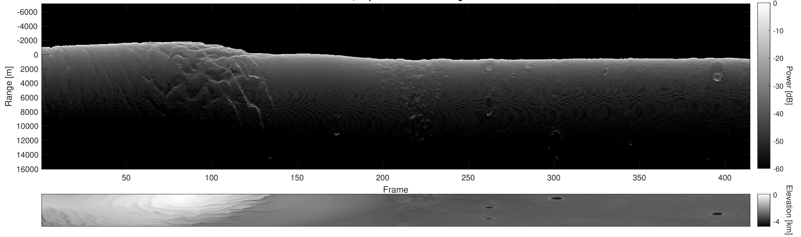
Orbit 5366, Depth-Corrected Cluttergram
