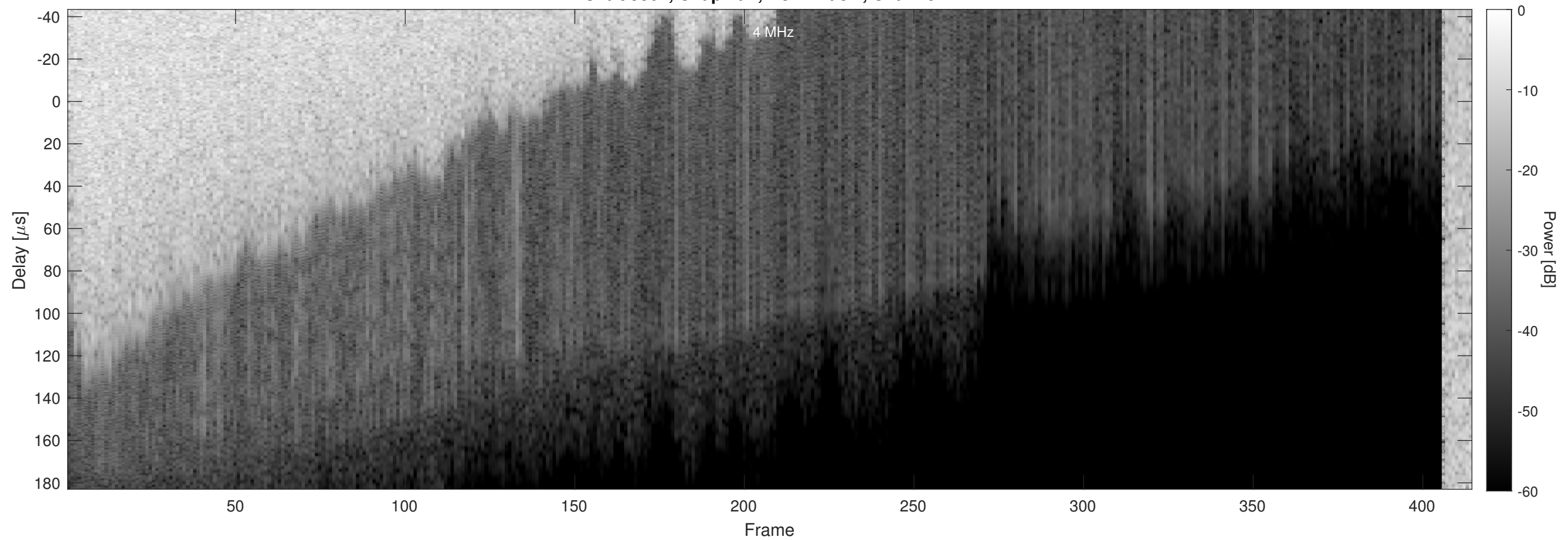
Orbit 5367, Chapman, No Window, Channel 2
