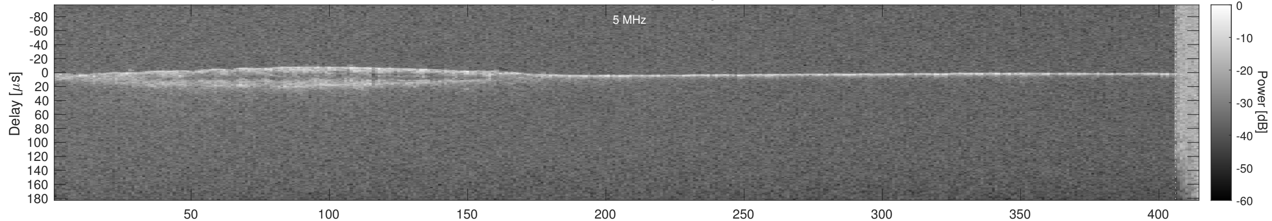
Orbit 5367, Cluttergram
