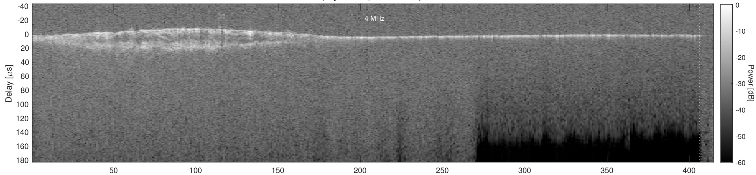
Orbit 5367, Cluttergram
