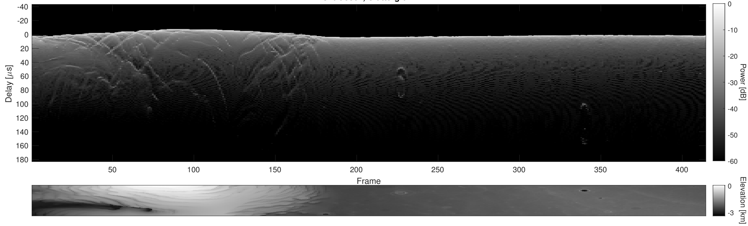
Orbit 5367, Cluttergram
