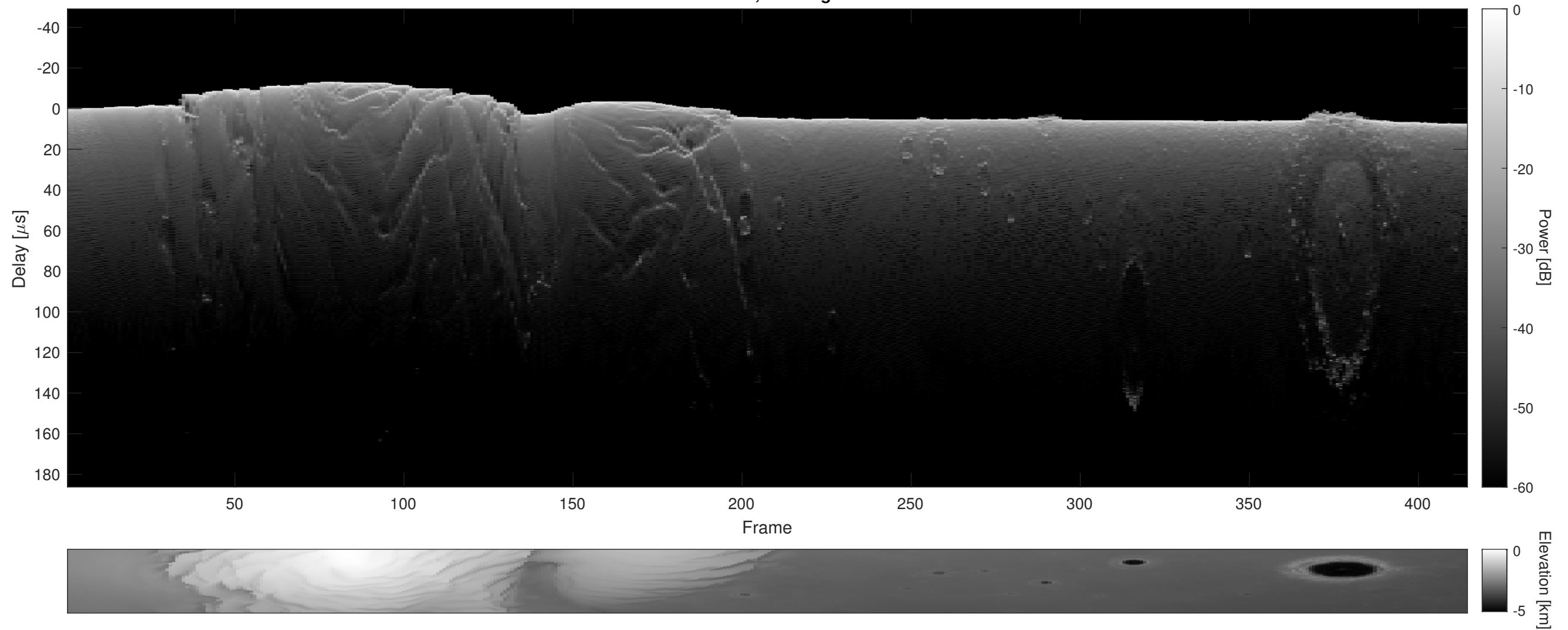
Orbit 5368, Cluttergram
