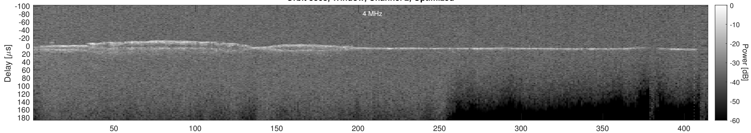
Orbit 5368, Cluttergram
