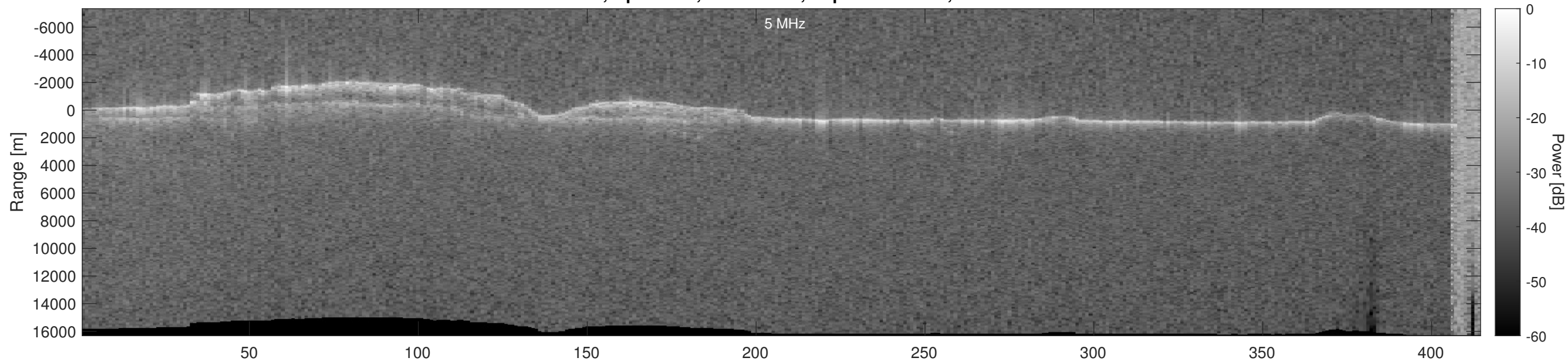
Orbit 5368, Optimized, No Window, Depth-Corrected, Channel 2
