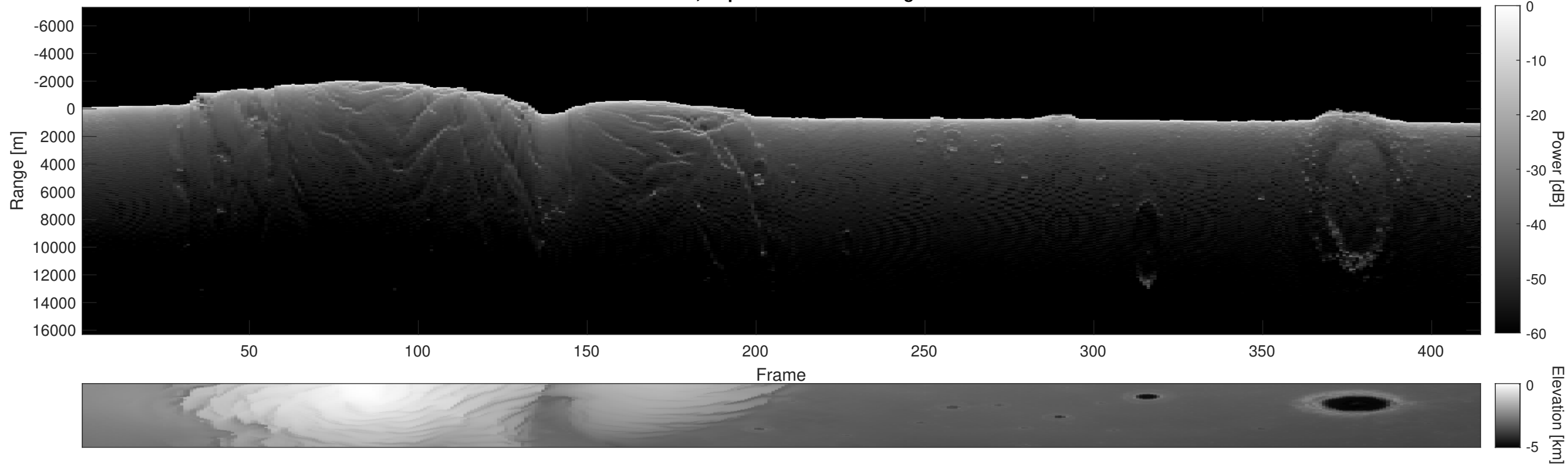
Orbit 5368, Depth-Corrected Cluttergram
