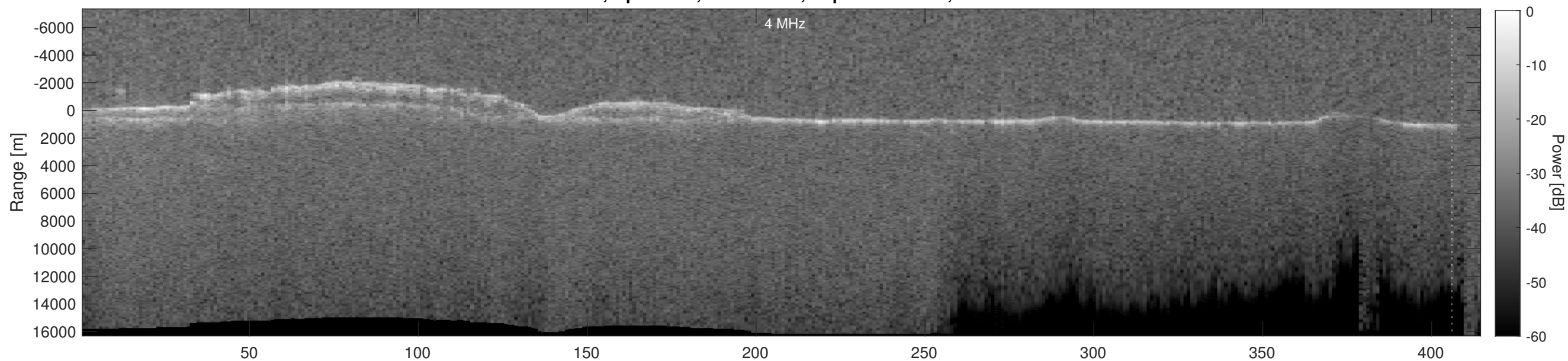
Orbit 5368, Depth-Corrected Cluttergram
