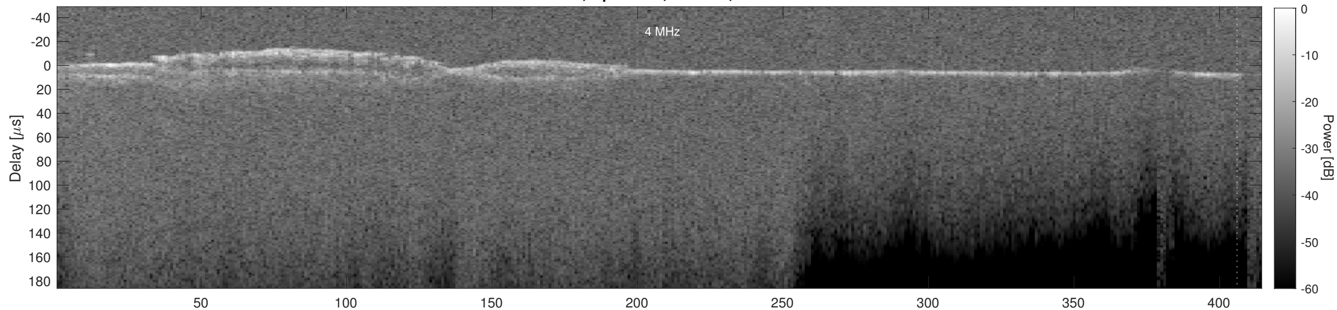
Orbit 5368, Cluttergram
