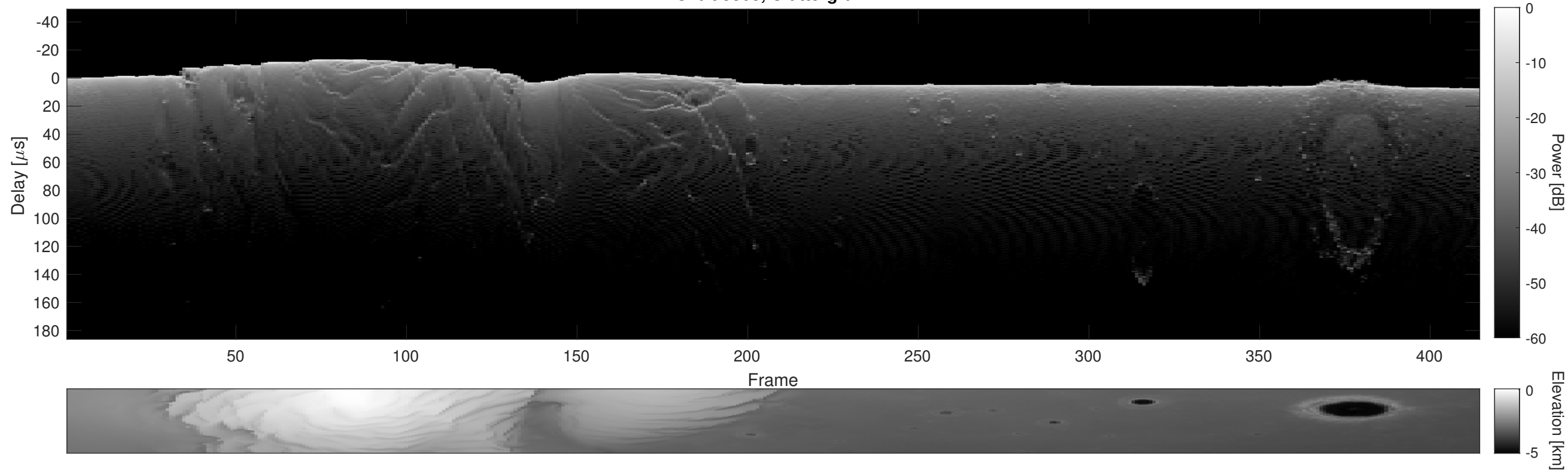
Orbit 5368, Cluttergram
