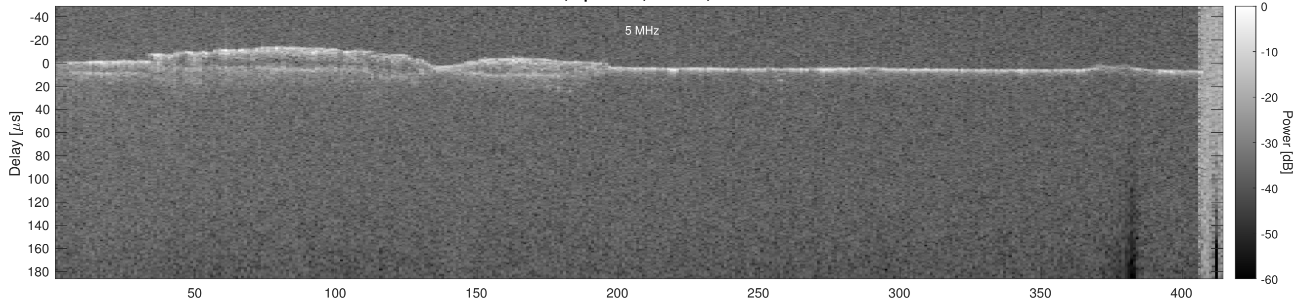
Orbit 5368, Optimized, Window, Channel 2
