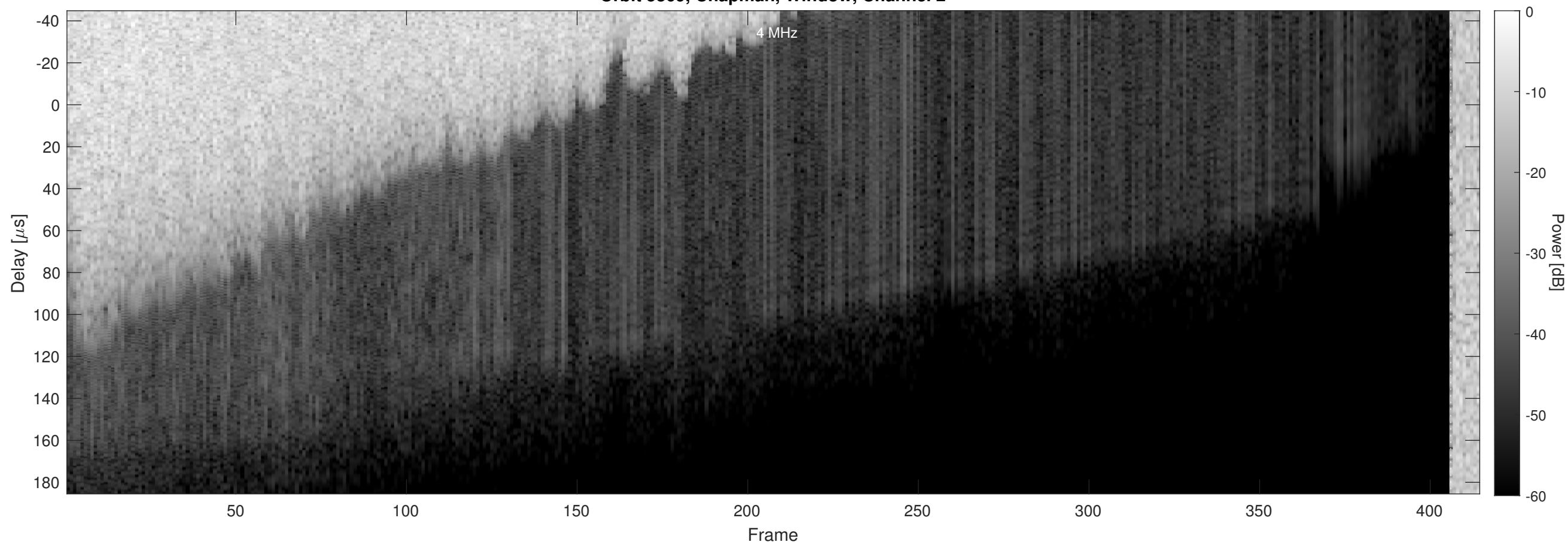
Orbit 5369, Chapman, Window, Channel 2
