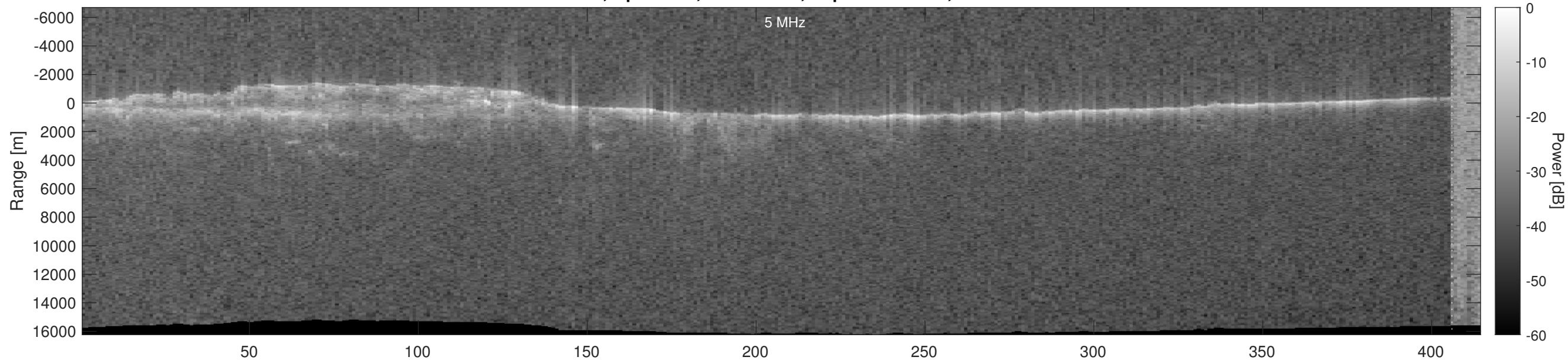
Orbit 5369, Optimized, No Window, Depth-Corrected, Channel 2
