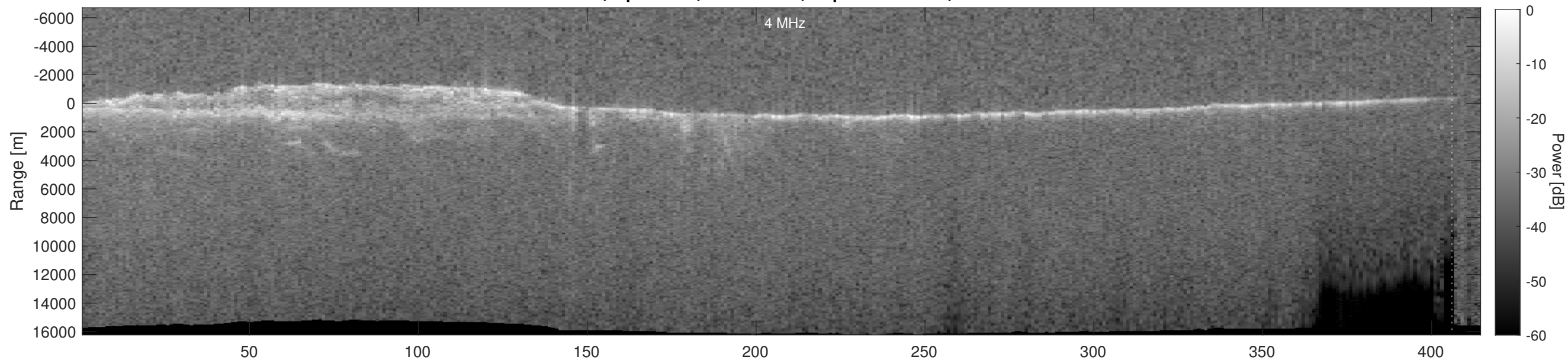
Orbit 5369, Depth-Corrected Cluttergram
