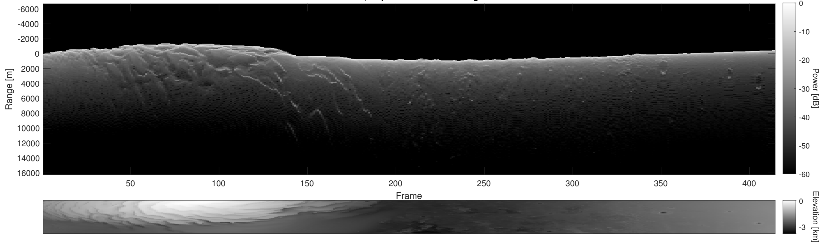
Orbit 5369, Depth-Corrected Cluttergram
