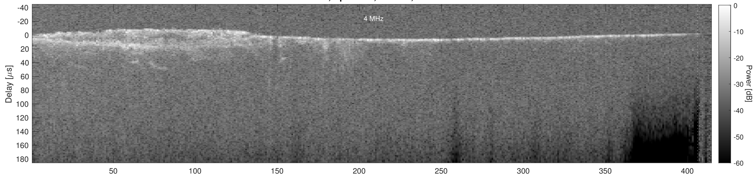
Orbit 5369, Cluttergram
