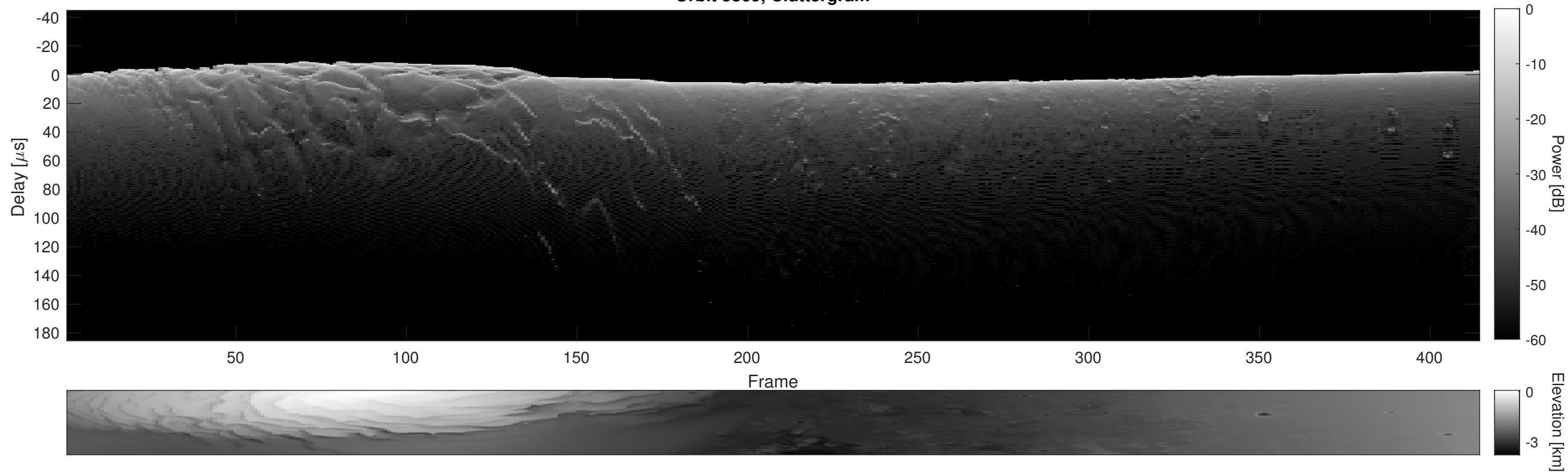
Orbit 5369, Cluttergram
