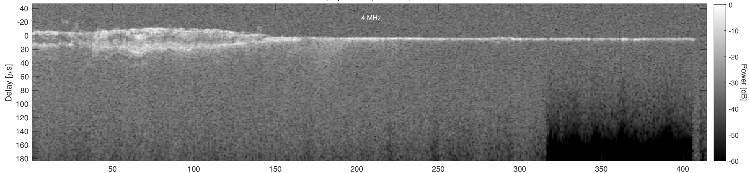
Orbit 5370, Cluttergram
