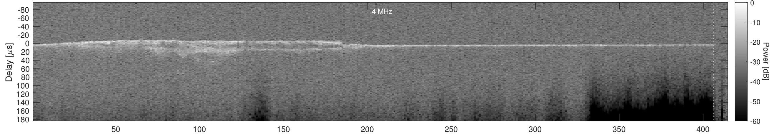
Orbit 5371, Cluttergram
