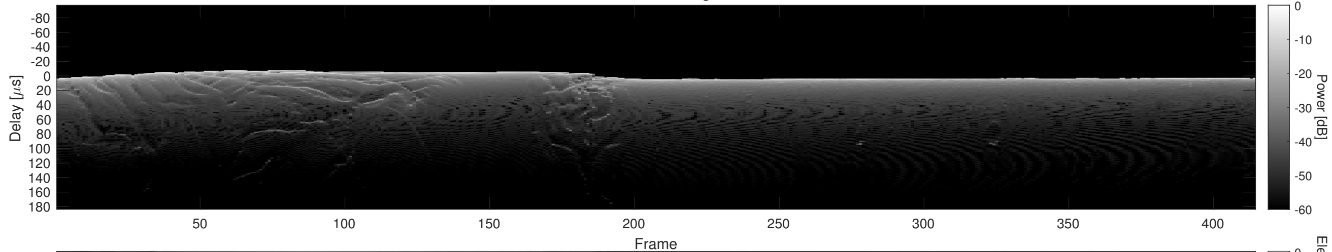
Orbit 5371, Cluttergram
