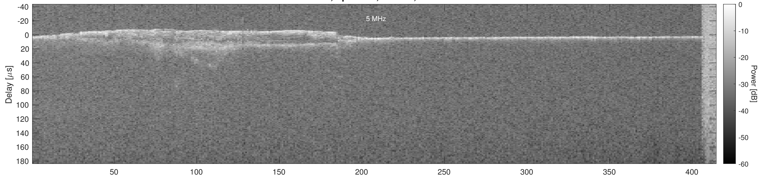
Orbit 5371, Optimized, Window, Channel 2
