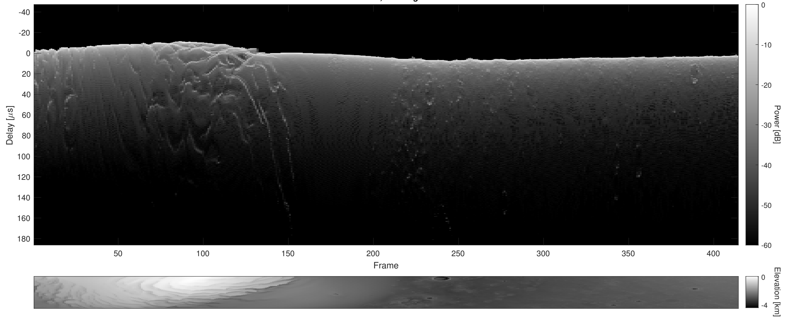
Orbit 5373, Cluttergram
