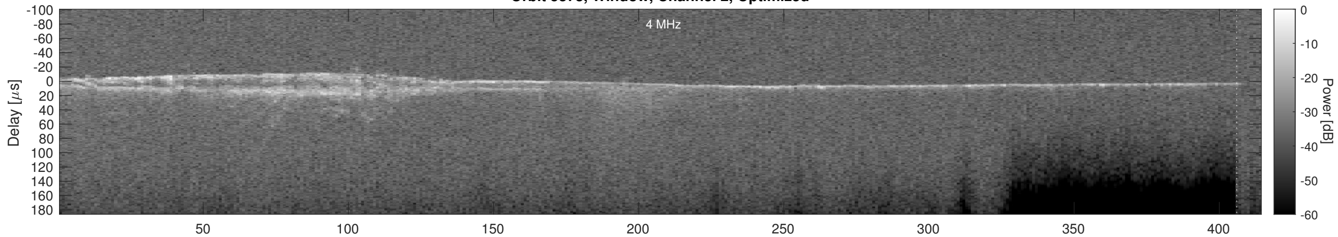
Orbit 5373, Cluttergram
