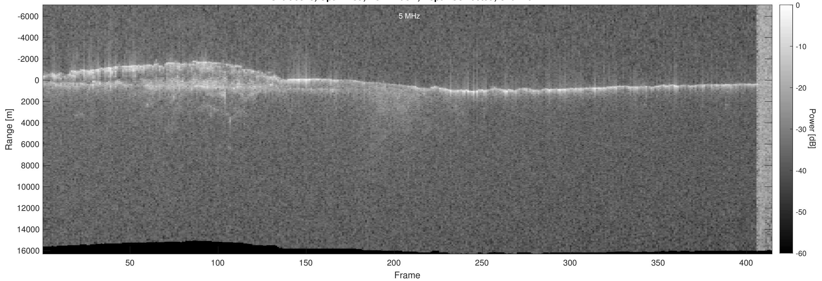
Orbit 5373, Optimized, No Window, Depth-Corrected, Channel 2
