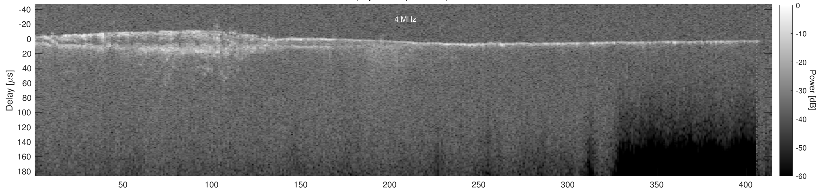
Orbit 5373, Cluttergram
