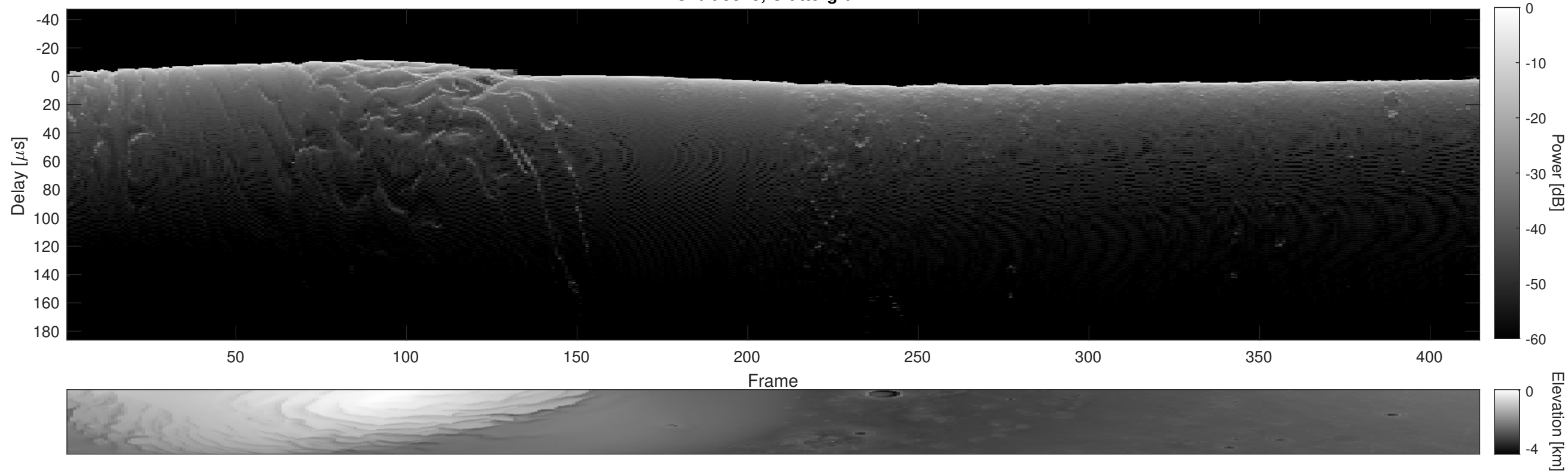
Orbit 5373, Cluttergram
