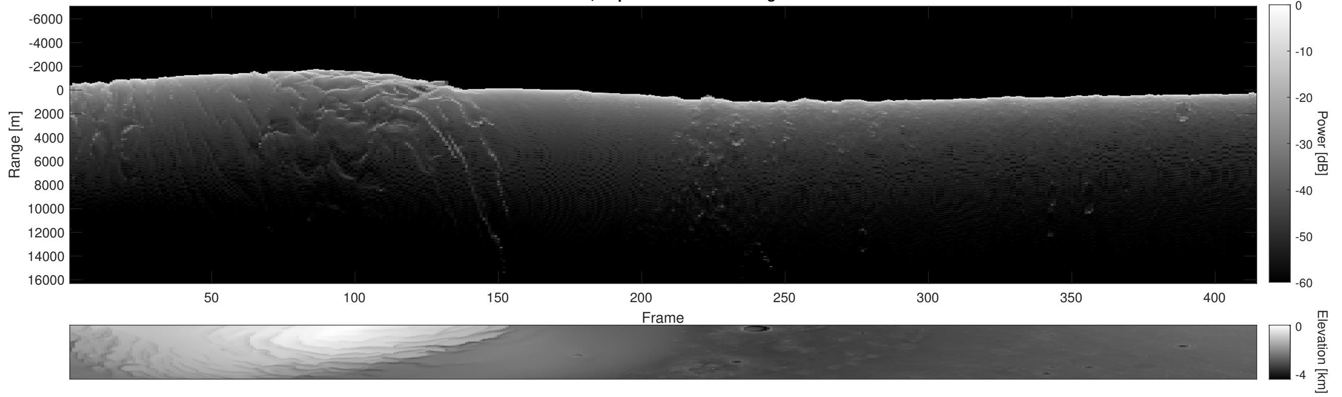
Orbit 5373, Depth-Corrected Cluttergram
