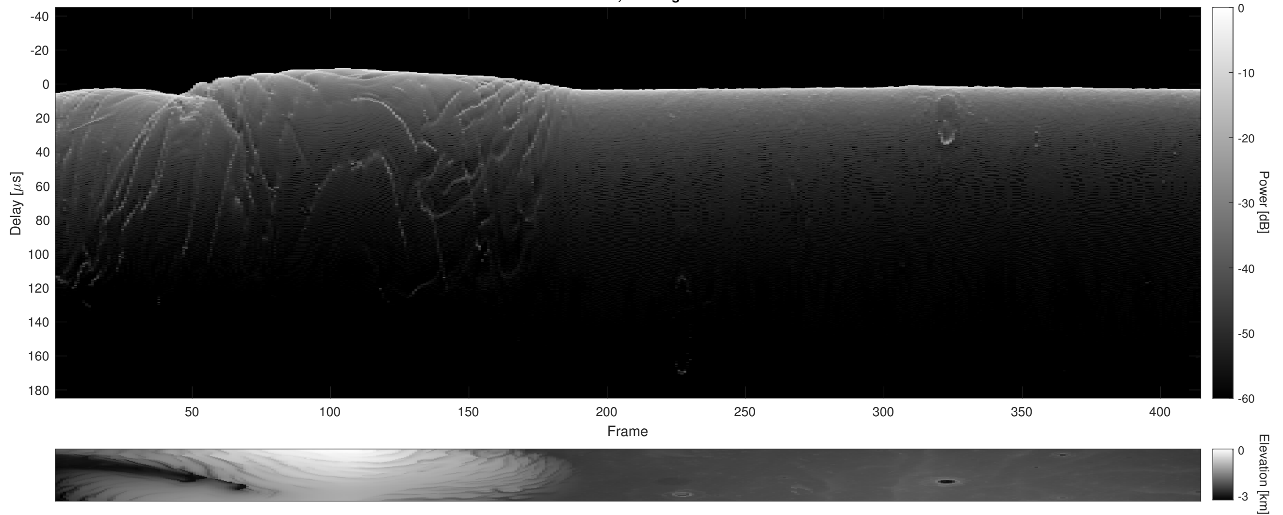
Orbit 5374, Cluttergram
