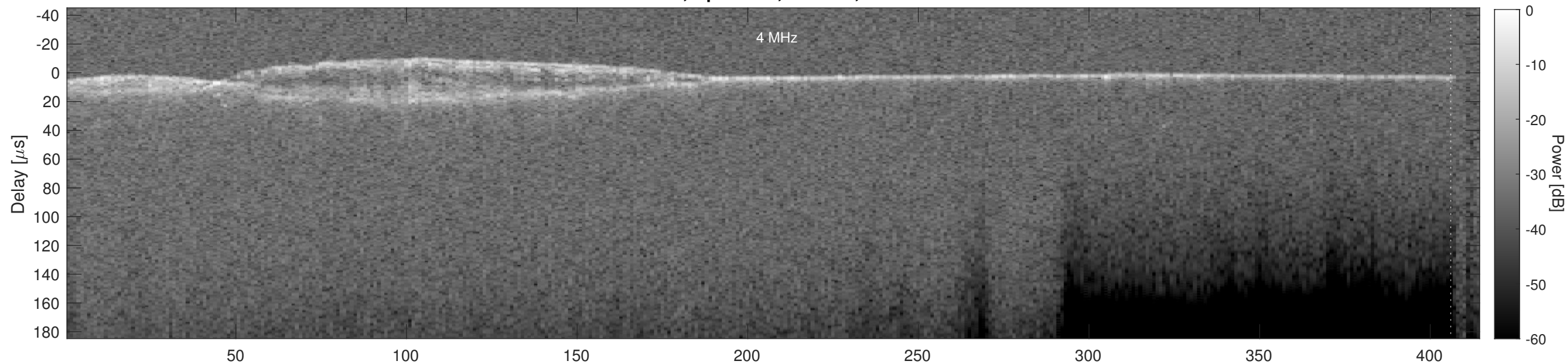
Orbit 5374, Cluttergram
