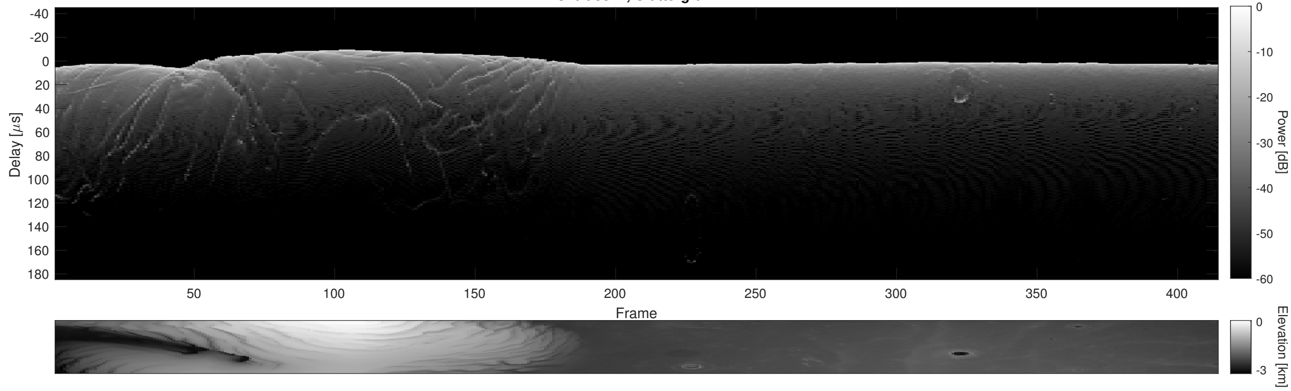
Orbit 5374, Cluttergram
