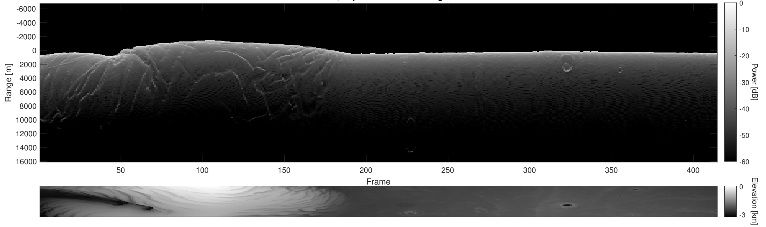
Orbit 5374, Depth-Corrected Cluttergram
