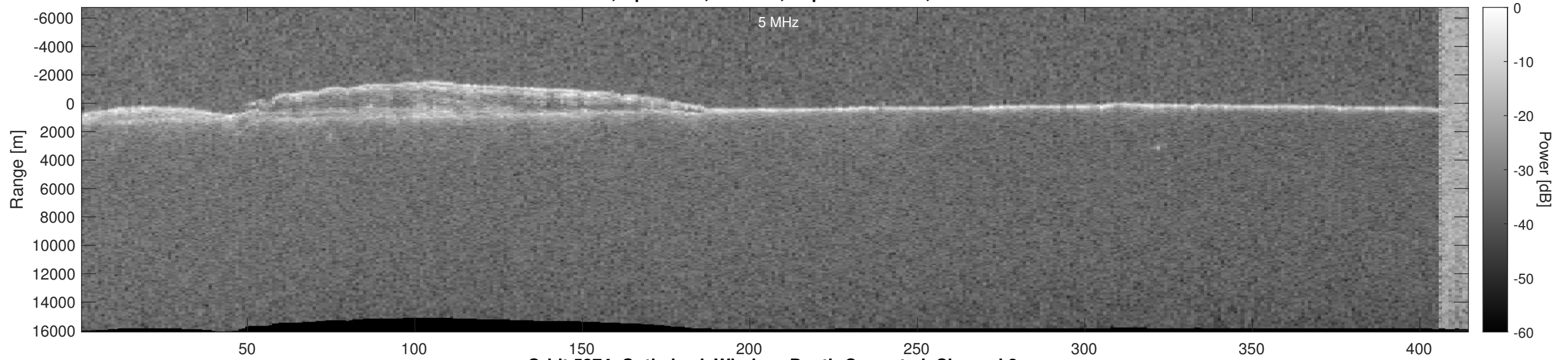
Orbit 5374, Optimized, Window, Depth-Corrected, Channel 2
