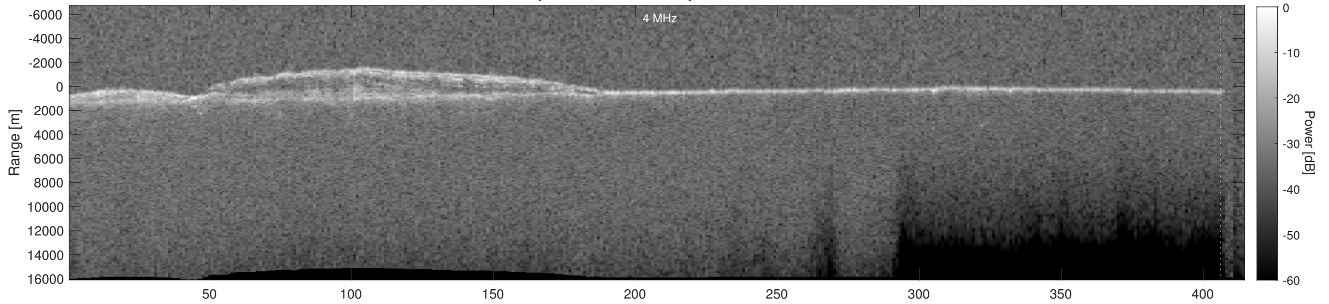
Orbit 5374, Depth-Corrected Cluttergram
