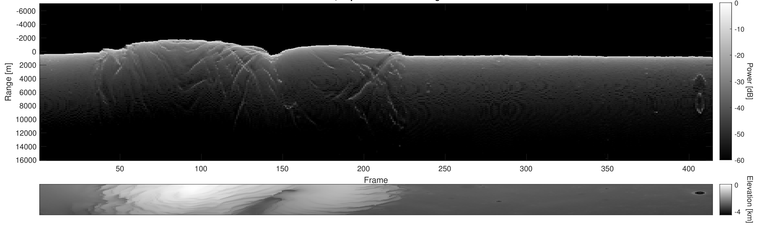
Orbit 5375, Depth-Corrected Cluttergram
