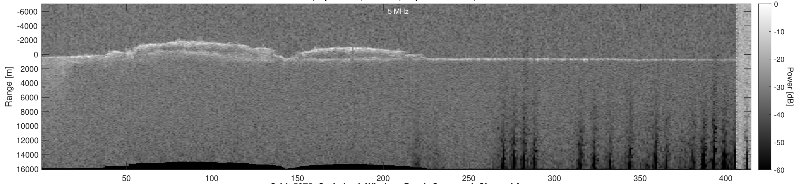
Orbit 5375, Optimized, Window, Depth-Corrected, Channel 2
