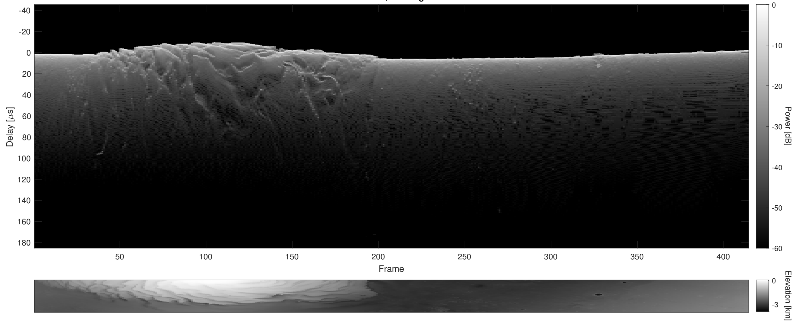
Orbit 5376, Cluttergram
