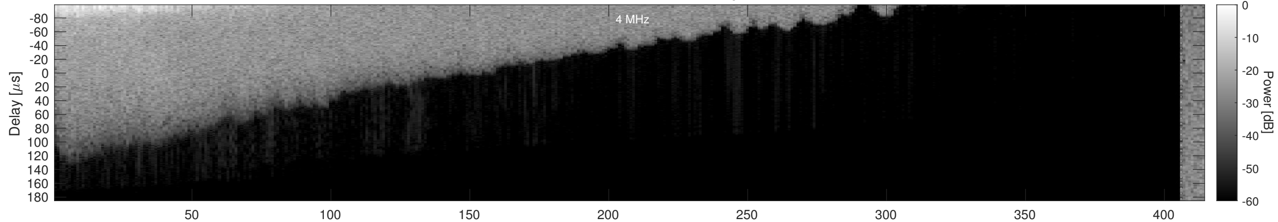
Orbit 5376, Window, Channel 2, Optimized
