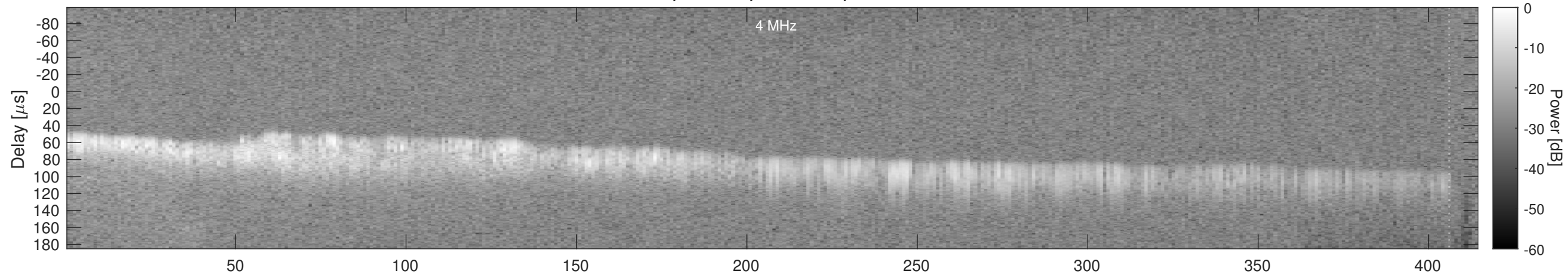
Orbit 5376, Window, Channel 2, Chapman
