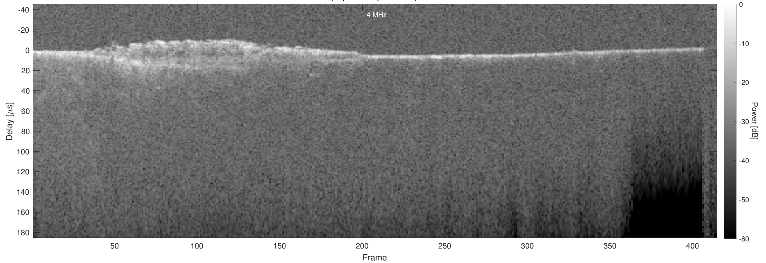
Orbit 5376, Optimized, Window, Channel 2
