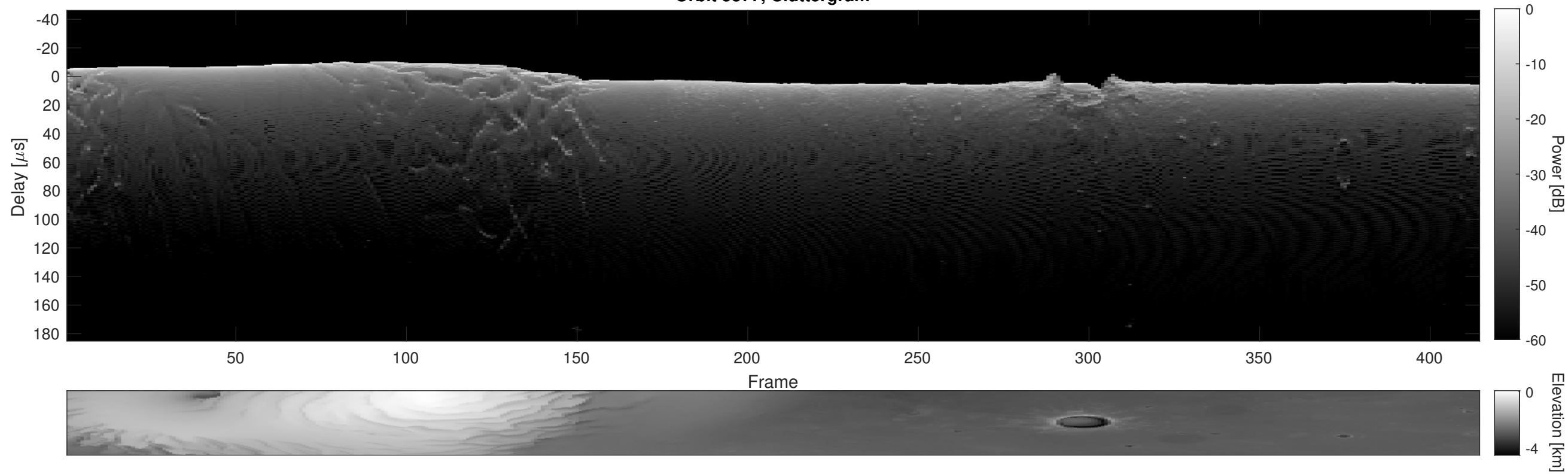
Orbit 5377, Cluttergram
