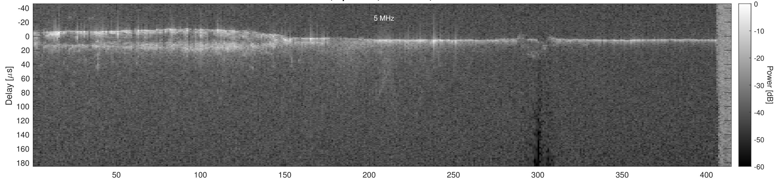
Orbit 5377, Optimized, No Window, Channel 2
