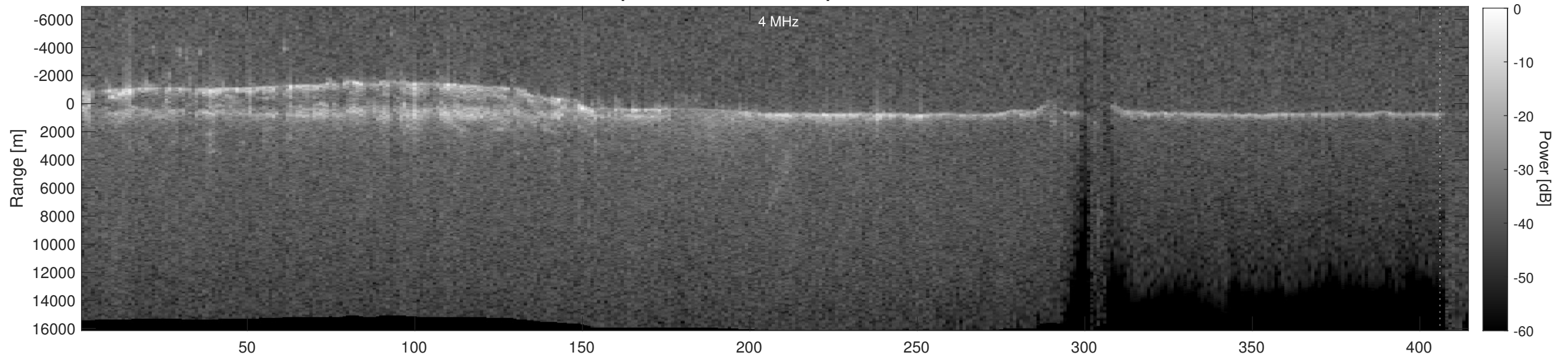
Orbit 5377, Depth-Corrected Cluttergram
