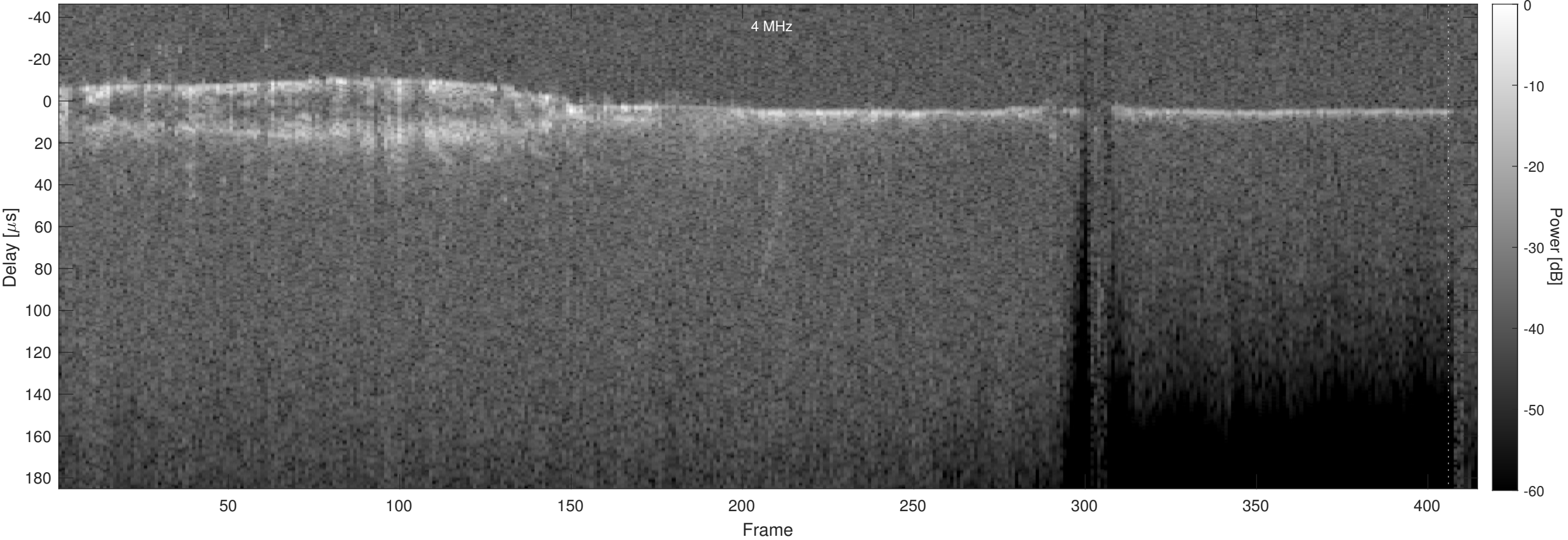
Orbit 5377, Optimized, Window, Channel 2
