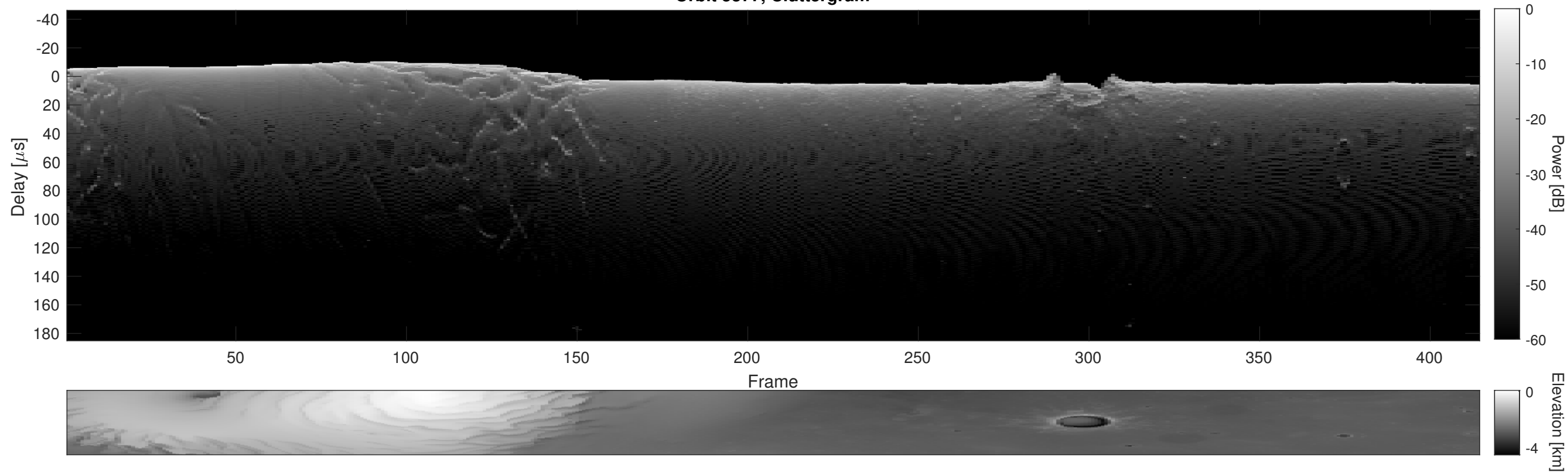
Orbit 5377, Cluttergram
