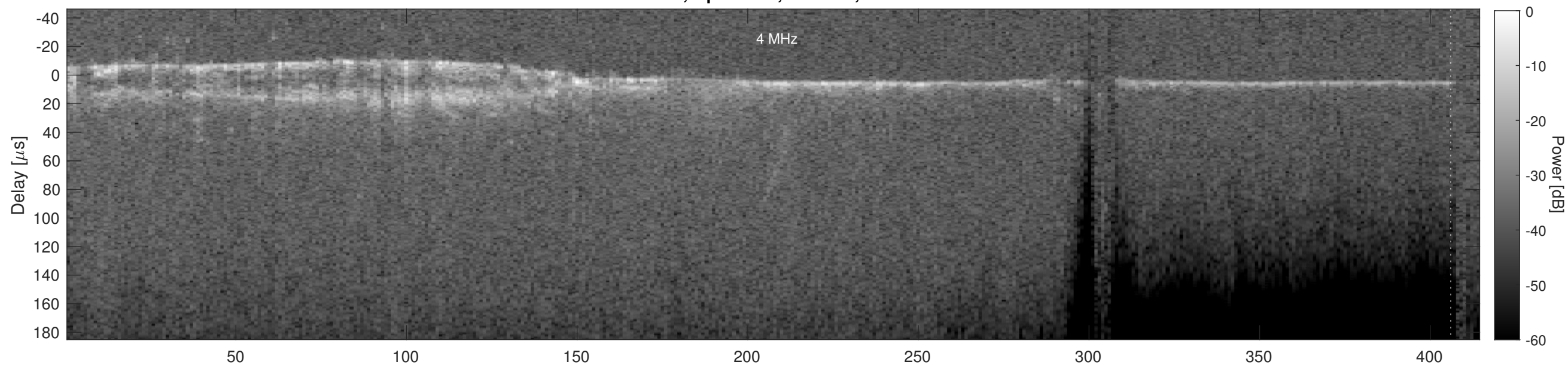
Orbit 5377, Cluttergram
