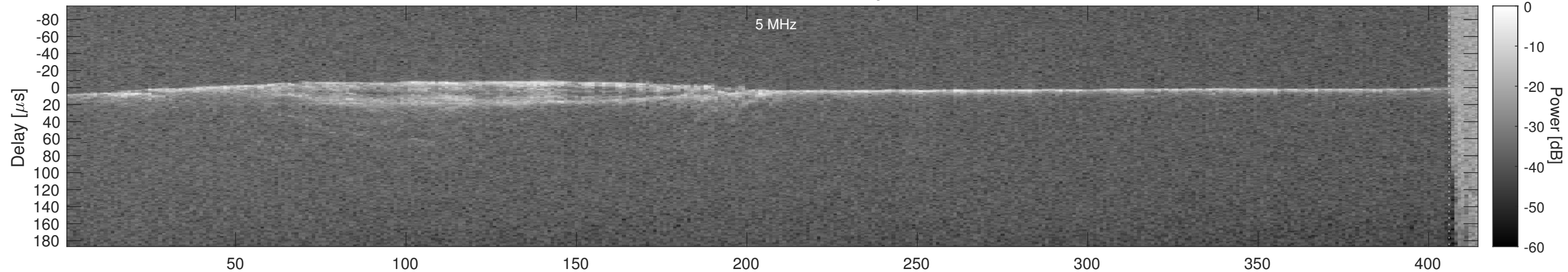
Orbit 5378, Cluttergram
