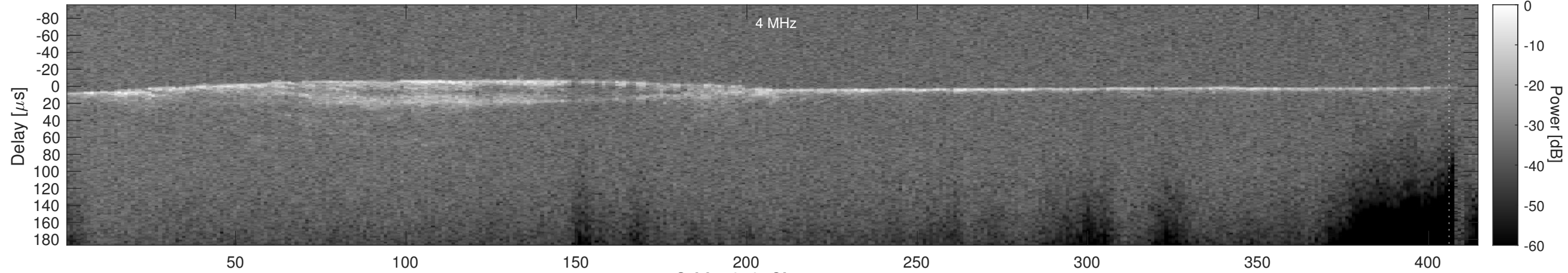
Orbit 5378, Cluttergram
