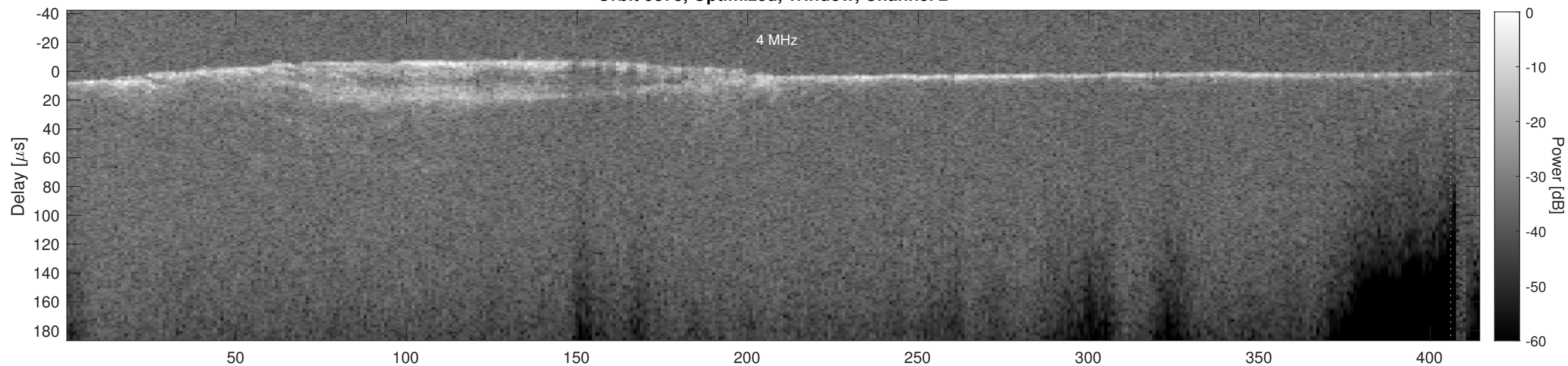
Orbit 5378, Cluttergram
