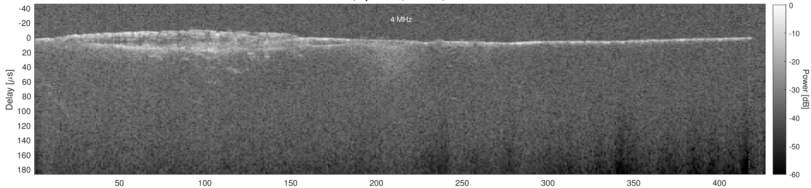
Orbit 5380, Cluttergram
