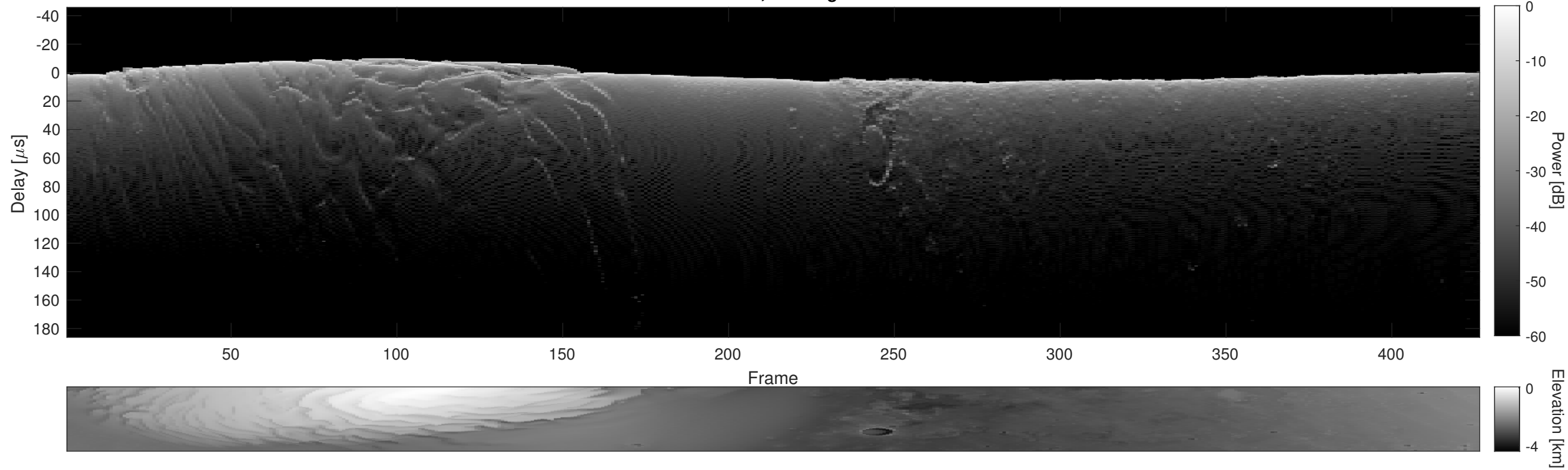
Orbit 5380, Cluttergram
