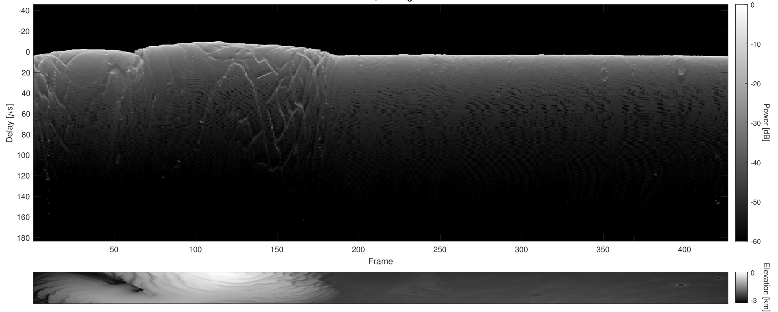
Orbit 5381, Cluttergram
