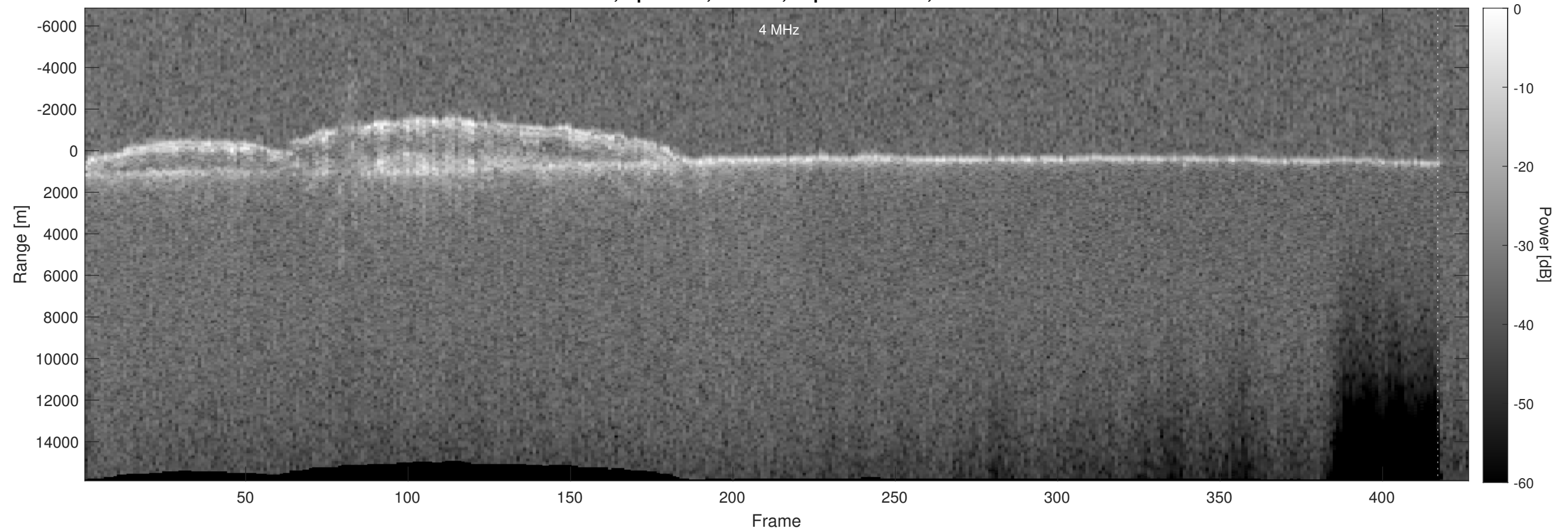
Orbit 5381, Optimized, Window, Depth-Corrected, Channel 2
